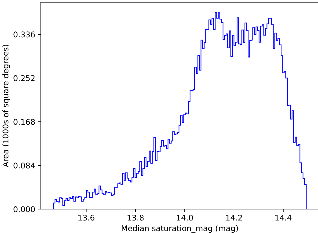
baseline_v2.0_10yrs All sky z band: Median saturation_mag
