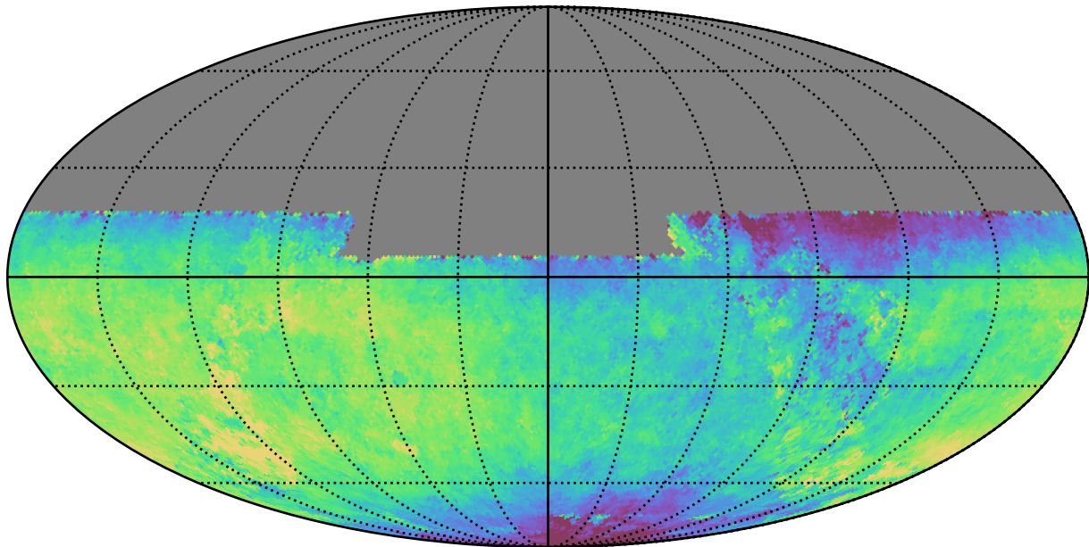
baseline_v2.0_10yrs All sky y band: Median saturation_mag
