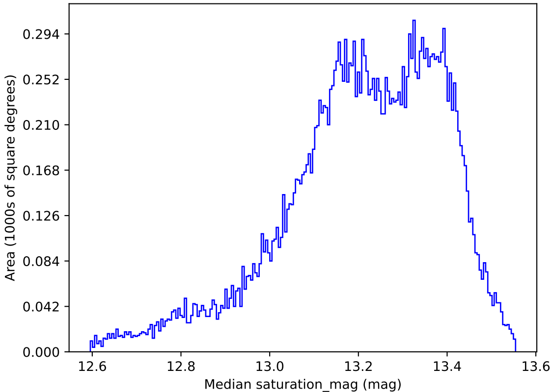
baseline_v2.0_10yrs All sky y band: Median saturation_mag
