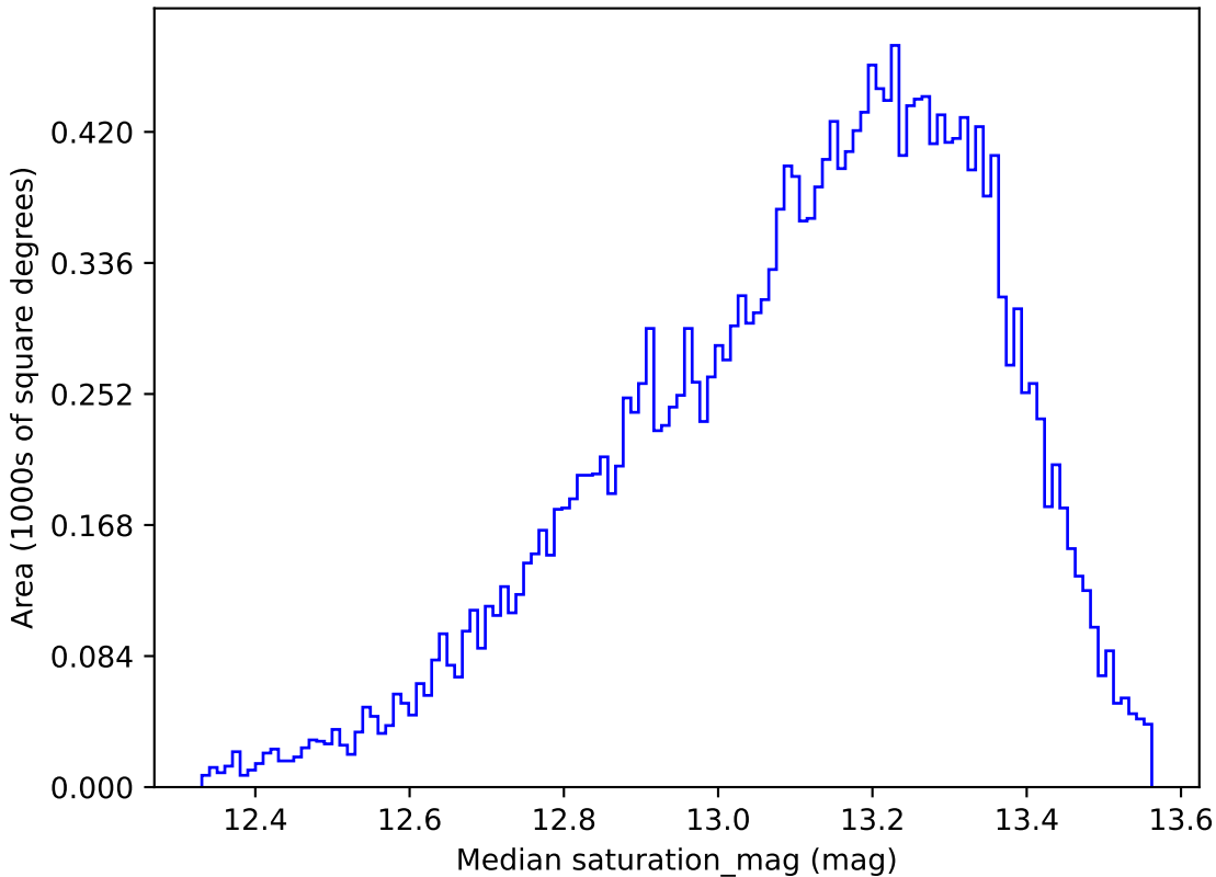
baseline_v2.0_10yrs All sky u band: Median saturation_mag
