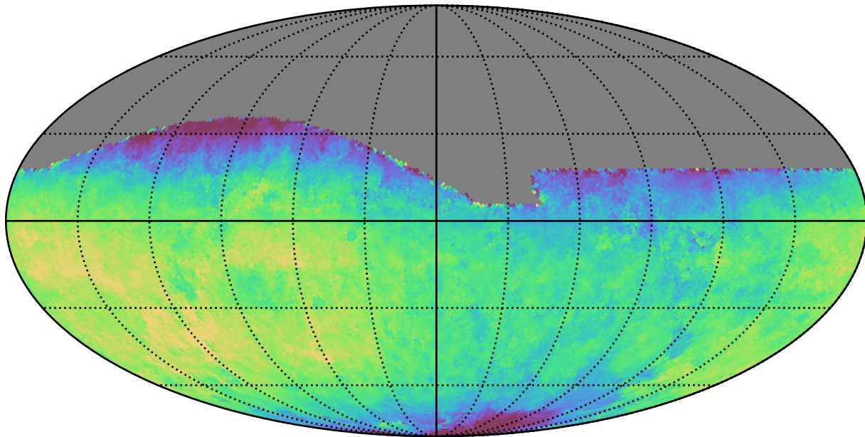
baseline_v2.0_10yrs All sky r band: Median saturation_mag
