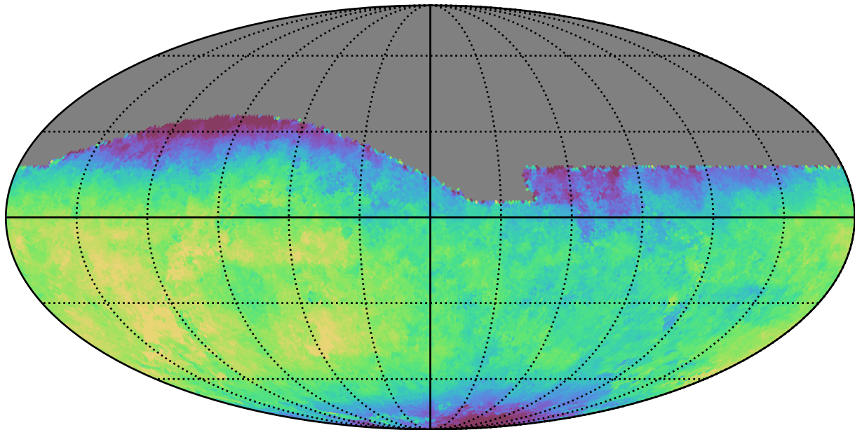
baseline_v2.0_10yrs All sky i band: Median saturation_mag
