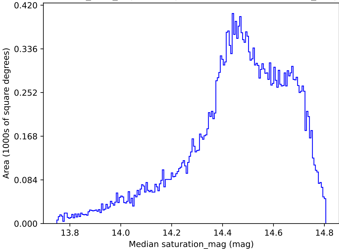
baseline_v2.0_10yrs All sky i band: Median saturation_mag
