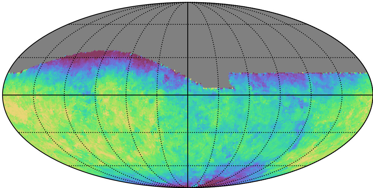
baseline_v2.0_10yrs All sky g band: Median saturation_mag
