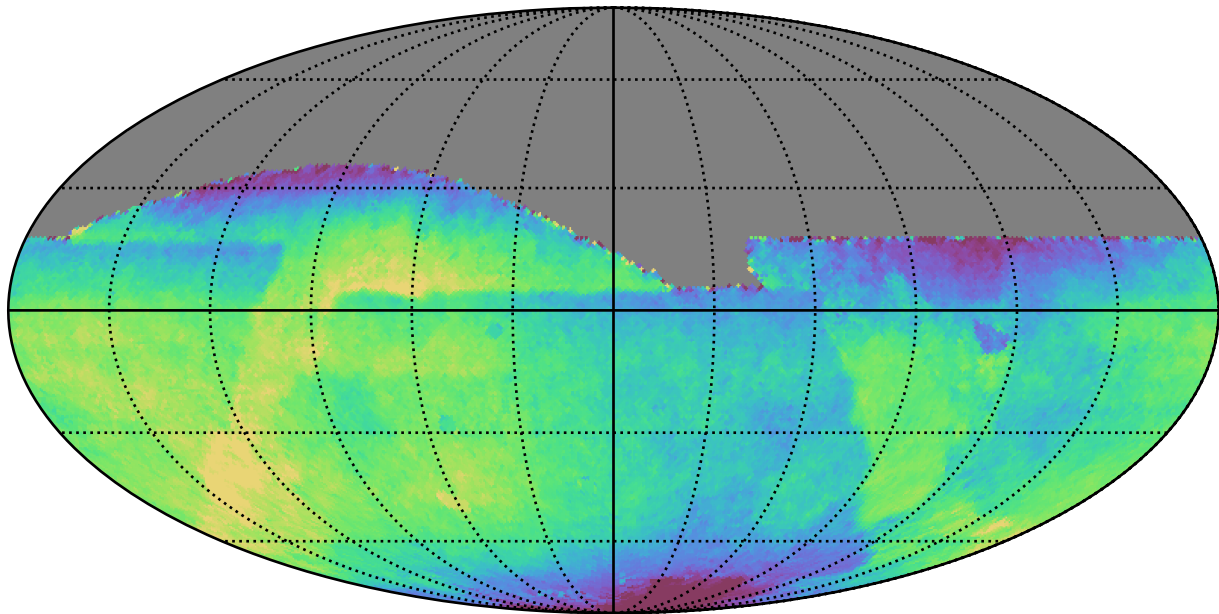
baseline_v2.0_10yrs All sky all bands: Median saturation_mag
