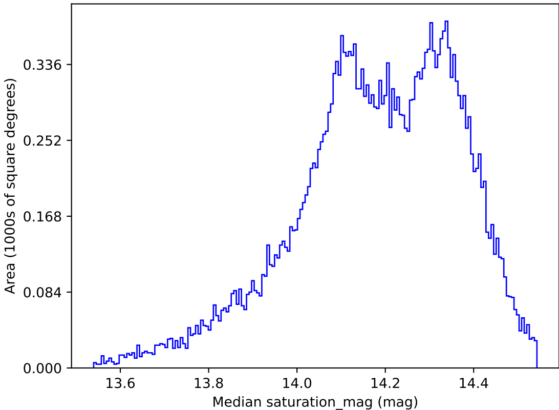
baseline_v2.0_10yrs All sky all bands: Median saturation_mag
