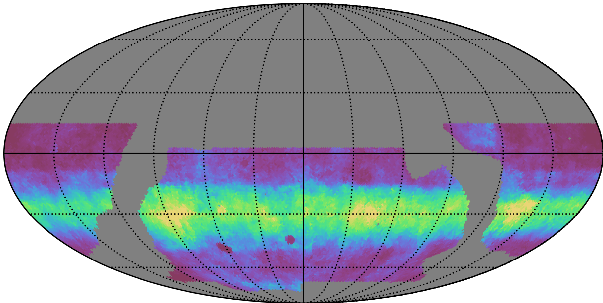
baseline_v2.0_10yrs WFD z band: Median normairmass
