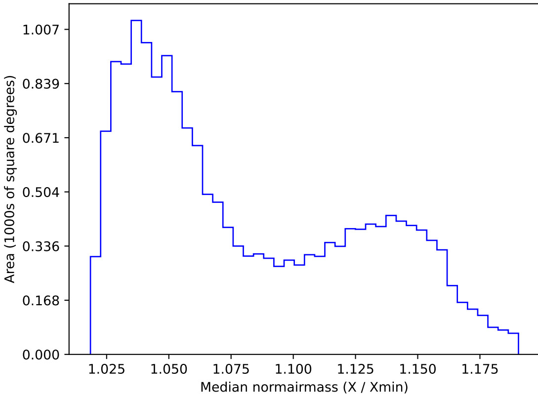
baseline_v2.0_10yrs WFD z band: Median normairmass
