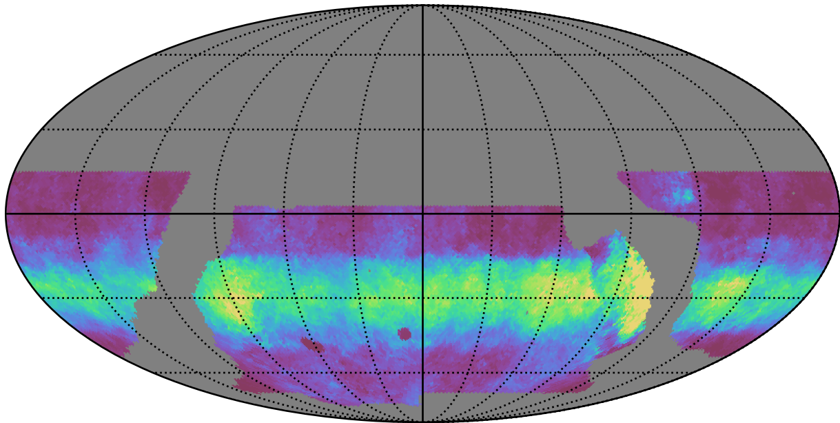
baseline_v2.0_10yrs WFD y band: Median normairmass
