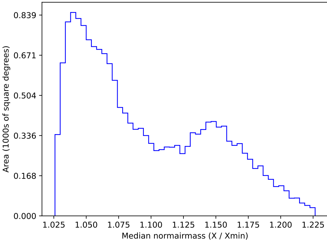
baseline_v2.0_10yrs WFD y band: Median normairmass
