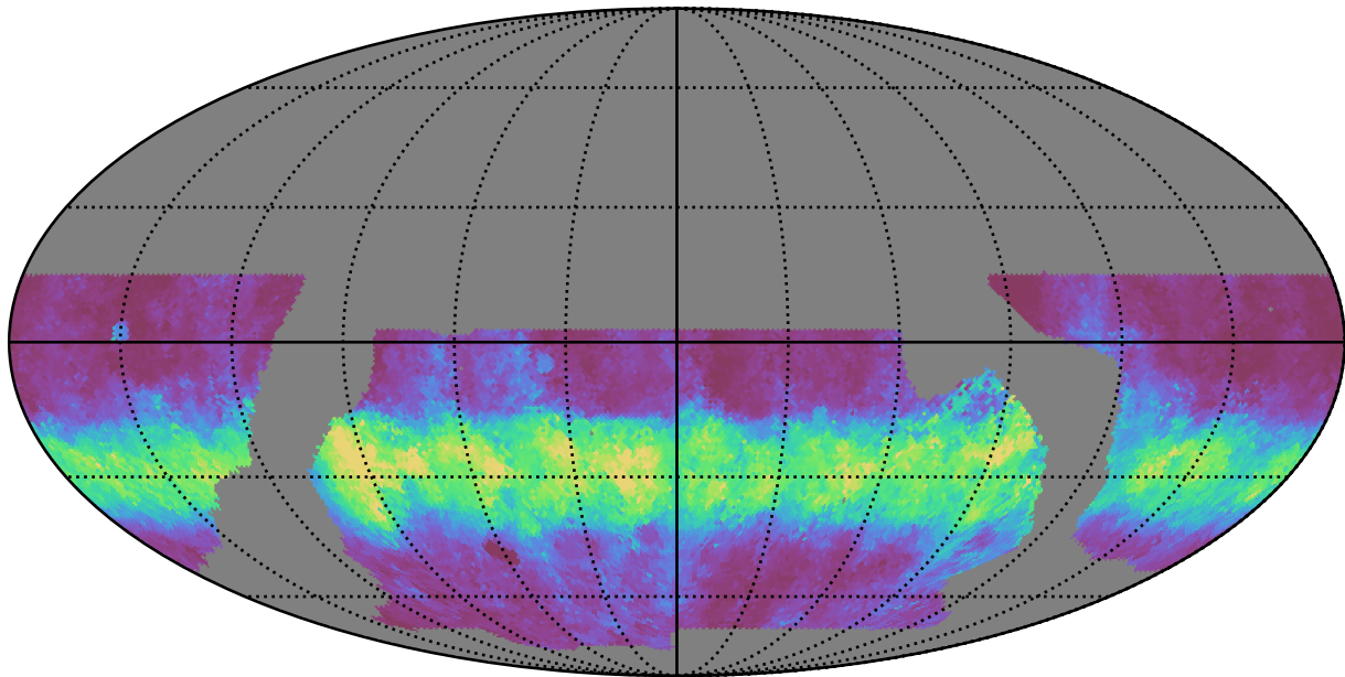
baseline_v2.0_10yrs WFD u band: Median normairmass
