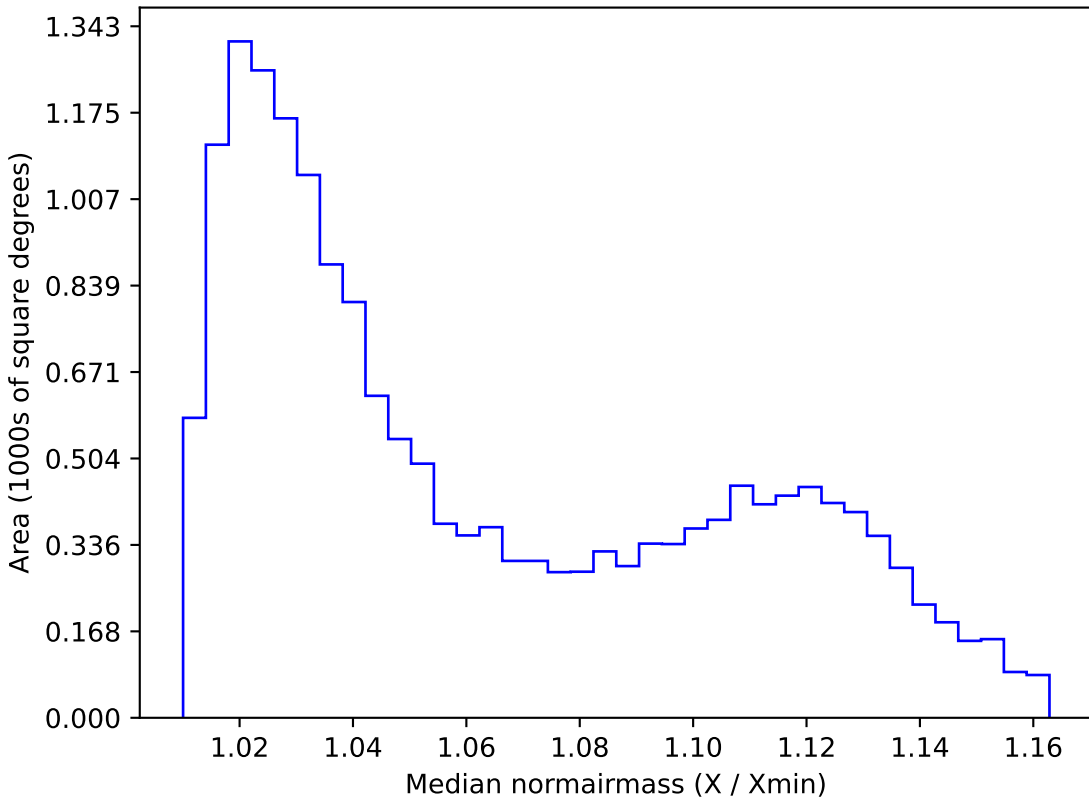
baseline_v2.0_10yrs WFD u band: Median normairmass
