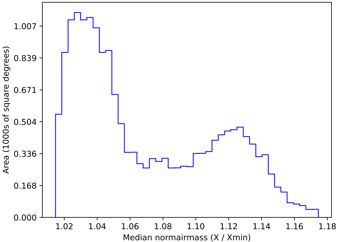
baseline_v2.0_10yrs WFD r band: Median normairmass
