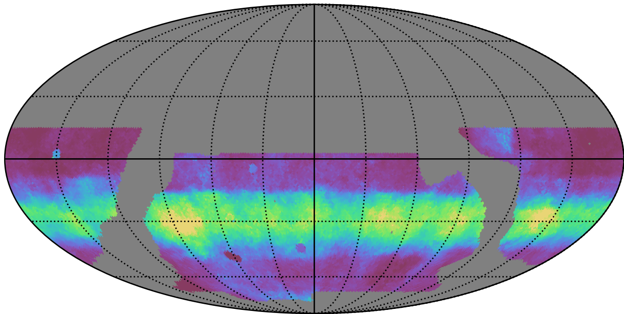
baseline_v2.0_10yrs WFD i band: Median normairmass
