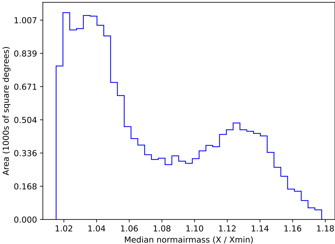
baseline_v2.0_10yrs WFD i band: Median normairmass
