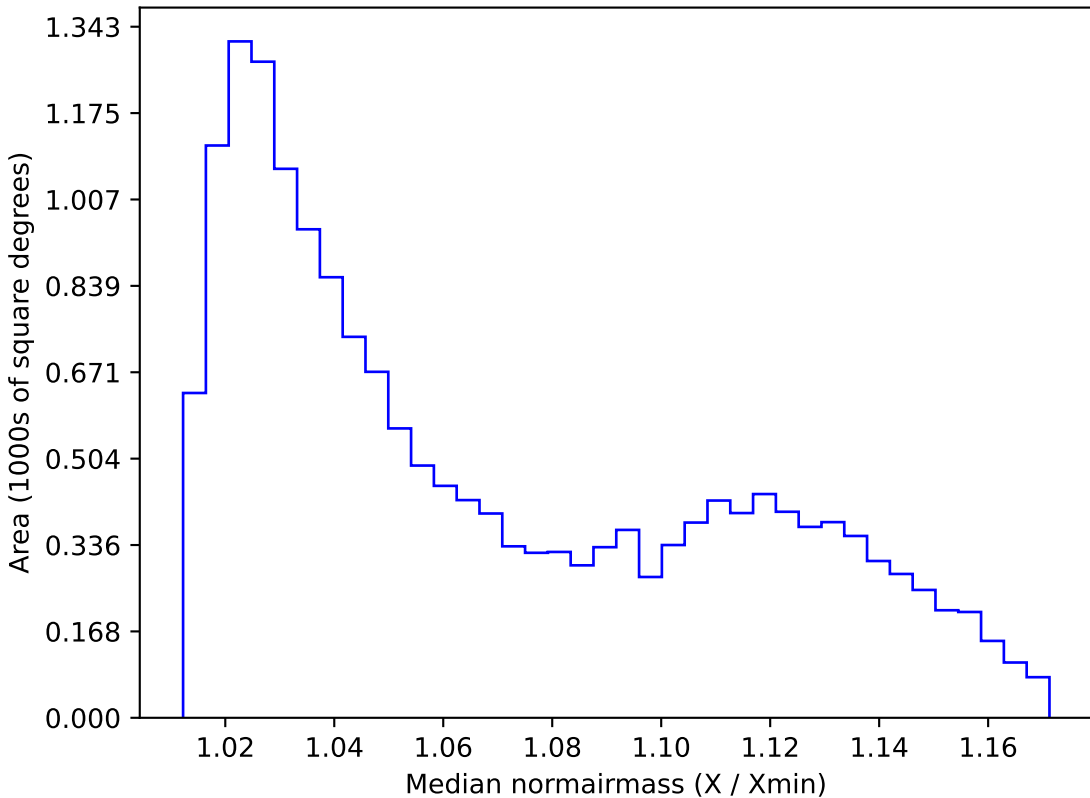
baseline_v2.0_10yrs WFD g band: Median normairmass
