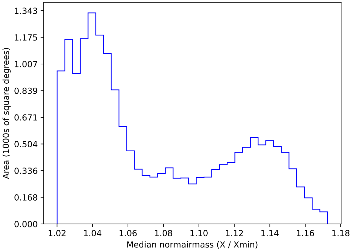
baseline_v2.0_10yrs WFD all bands: Median normairmass
