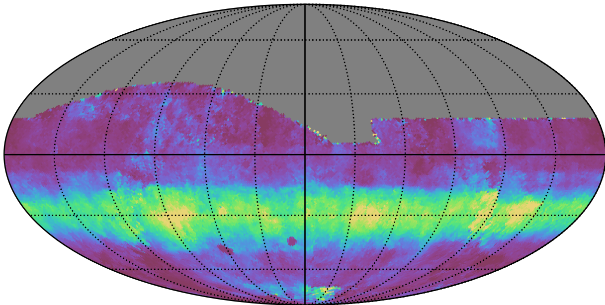
baseline_v2.0_10yrs All sky z band: Median normairmass
