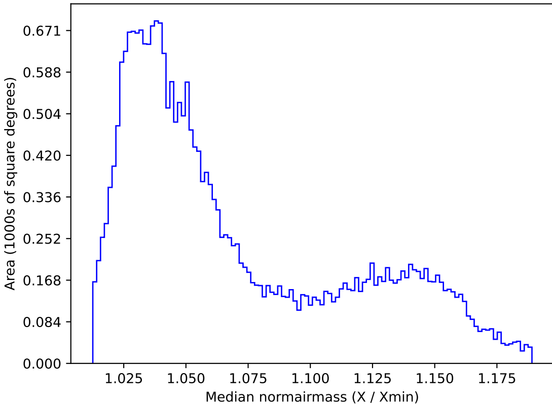
baseline_v2.0_10yrs All sky z band: Median normairmass
