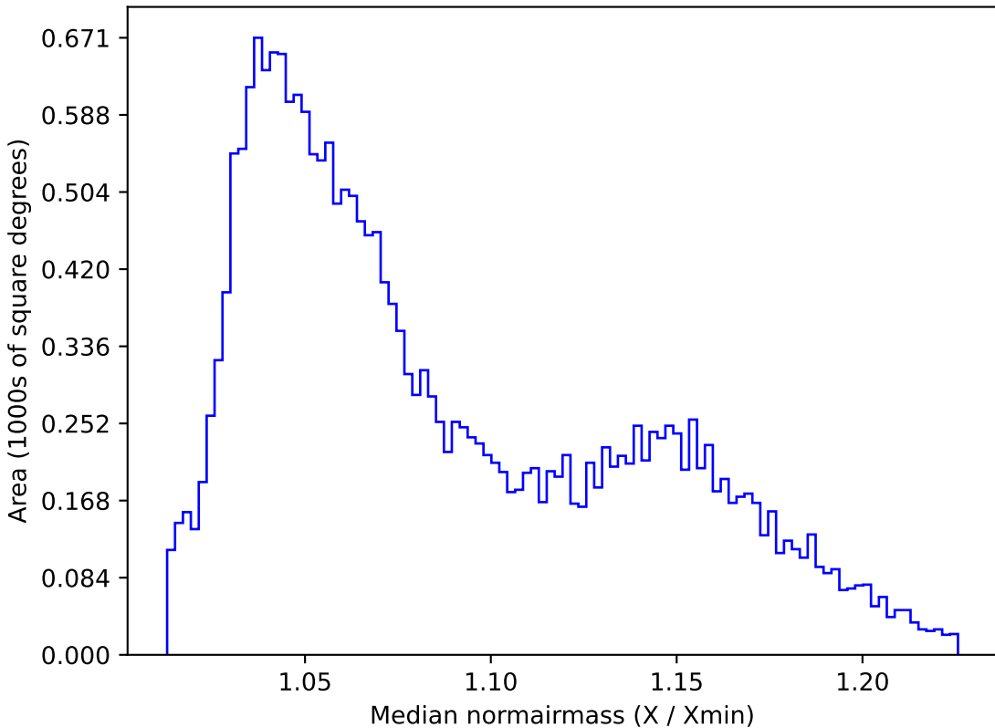
baseline_v2.0_10yrs All sky y band: Median normairmass
