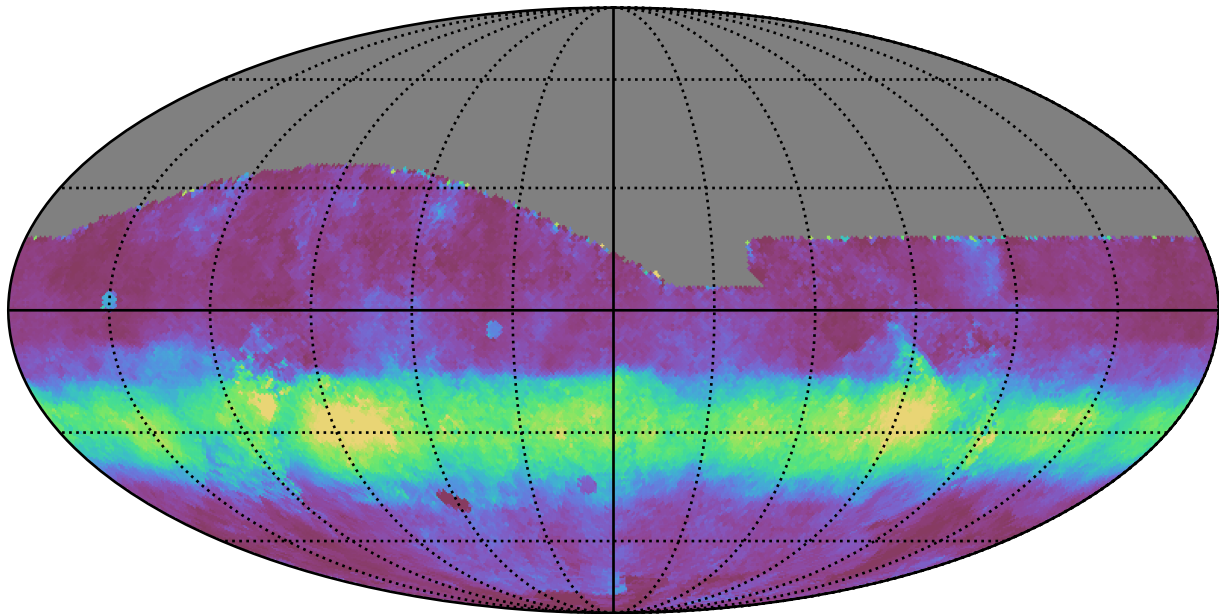
baseline_v2.0_10yrs All sky r band: Median normairmass
