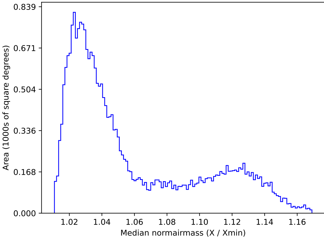
baseline_v2.0_10yrs All sky r band: Median normairmass
