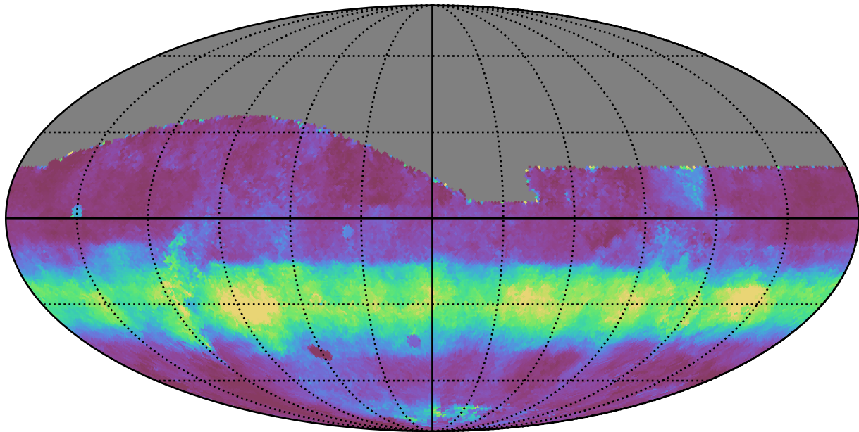
baseline_v2.0_10yrs All sky i band: Median normairmass
