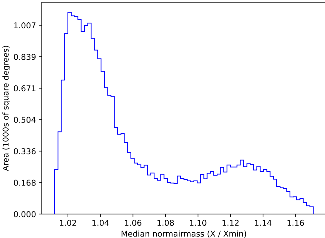
baseline_v2.0_10yrs All sky i band: Median normairmass
