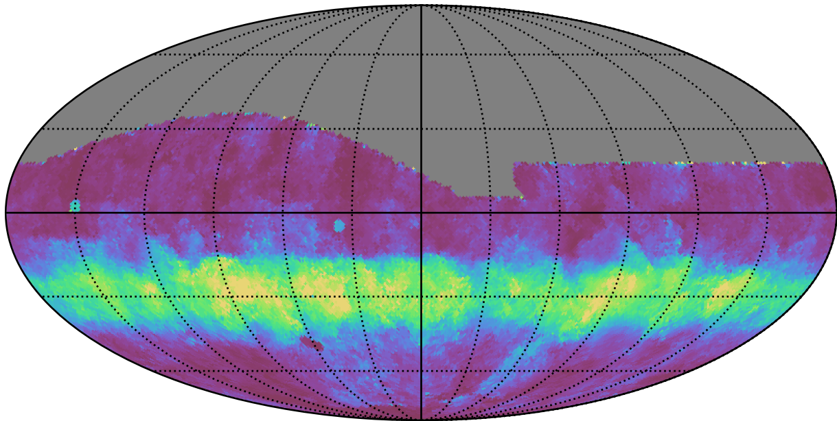
baseline_v2.0_10yrs All sky g band: Median normairmass
