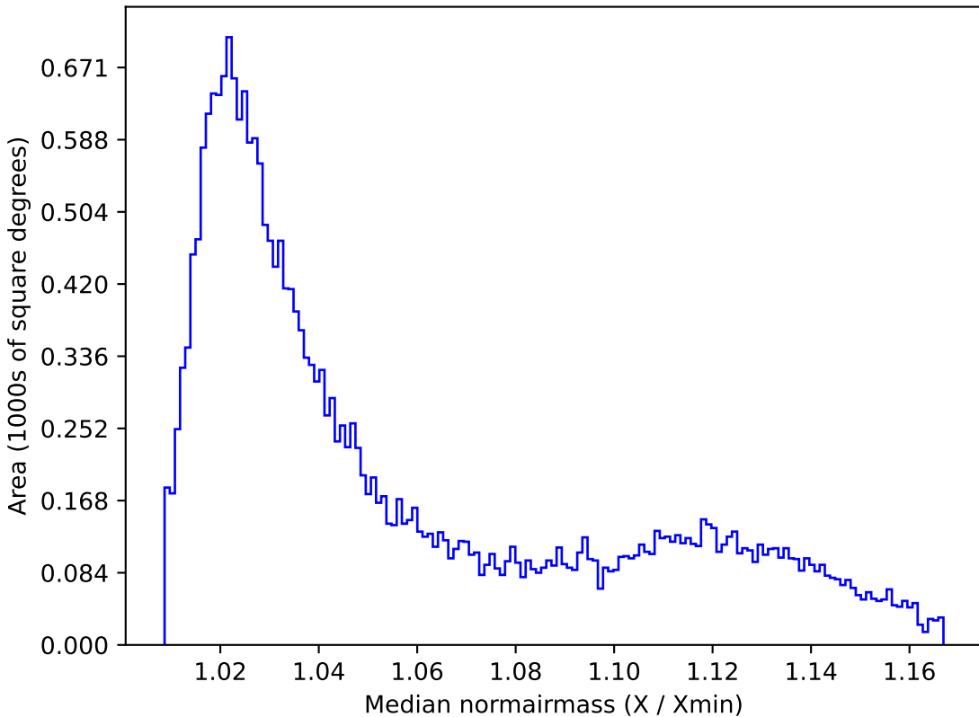
baseline_v2.0_10yrs All sky g band: Median normairmass
