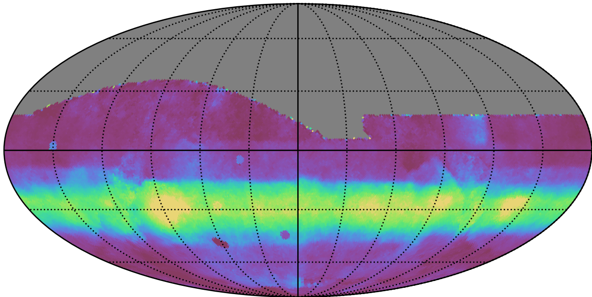
baseline_v2.0_10yrs All sky all bands: Median normairmass
