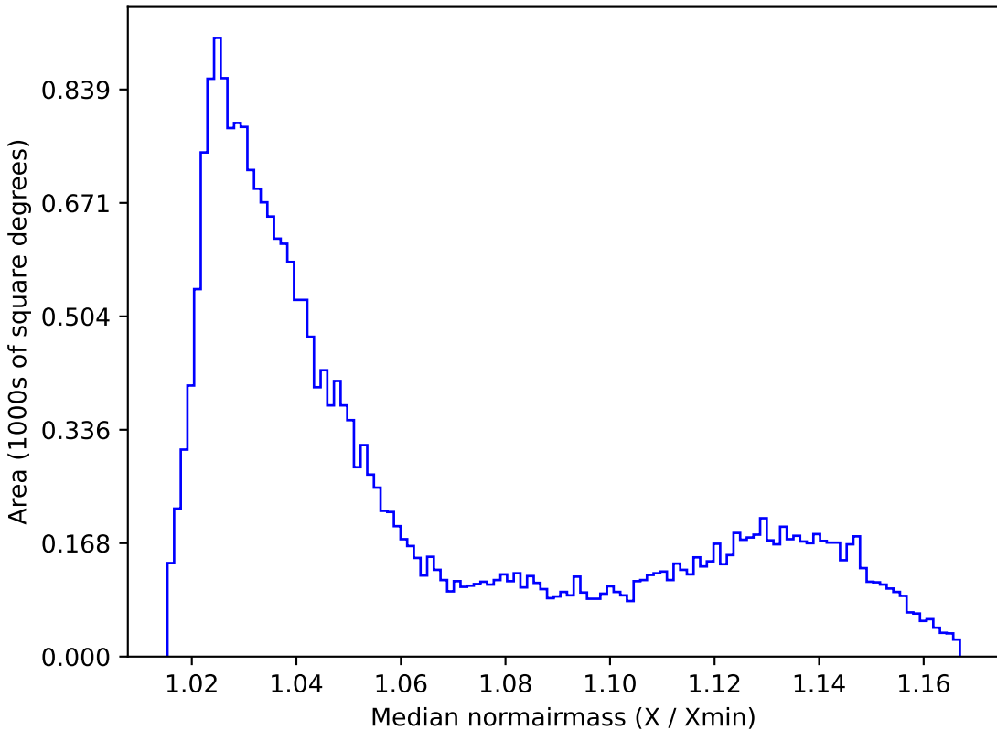
baseline_v2.0_10yrs All sky all bands: Median normairmass
