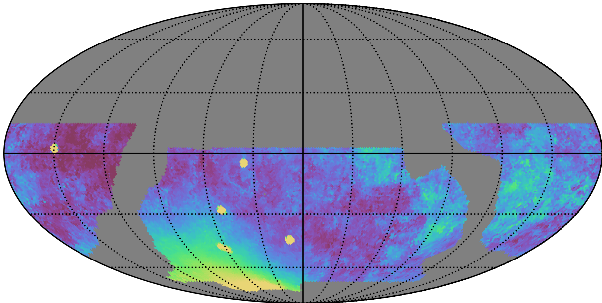
baseline_v2.0_10yrs WFD z band: Median moonDistance
