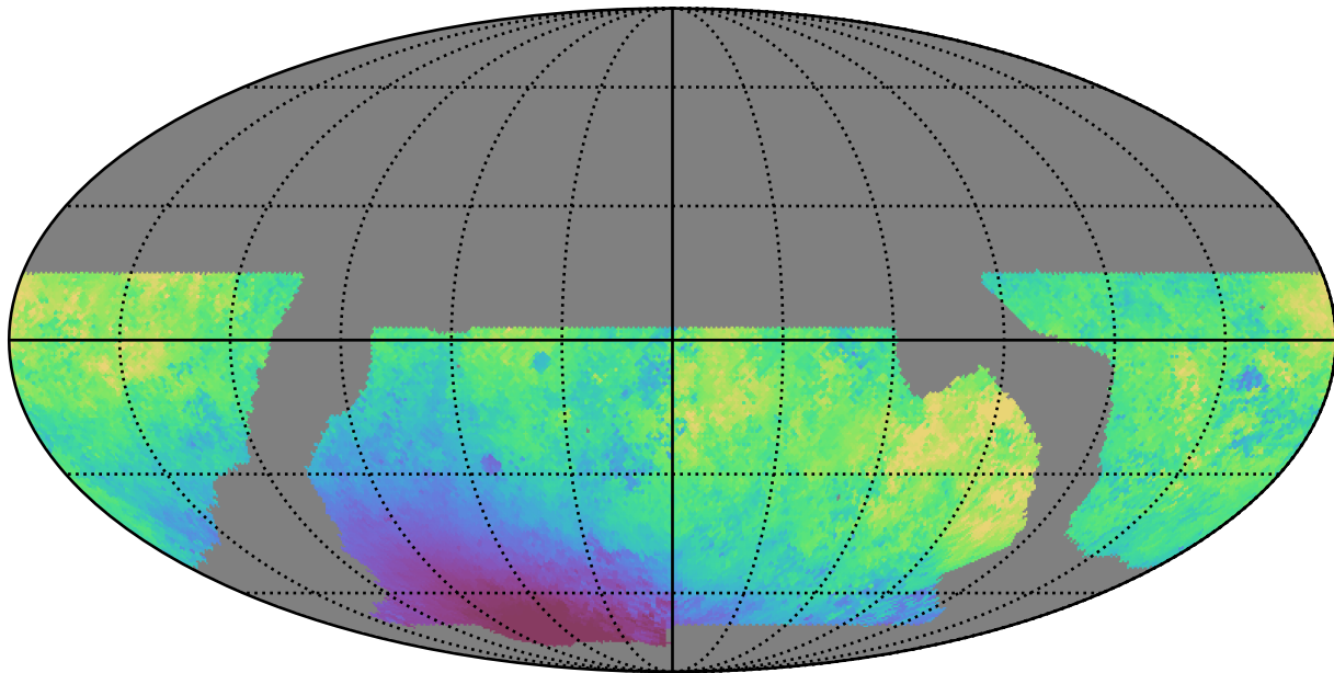
baseline_v2.0_10yrs WFD u band: Median moonDistance
