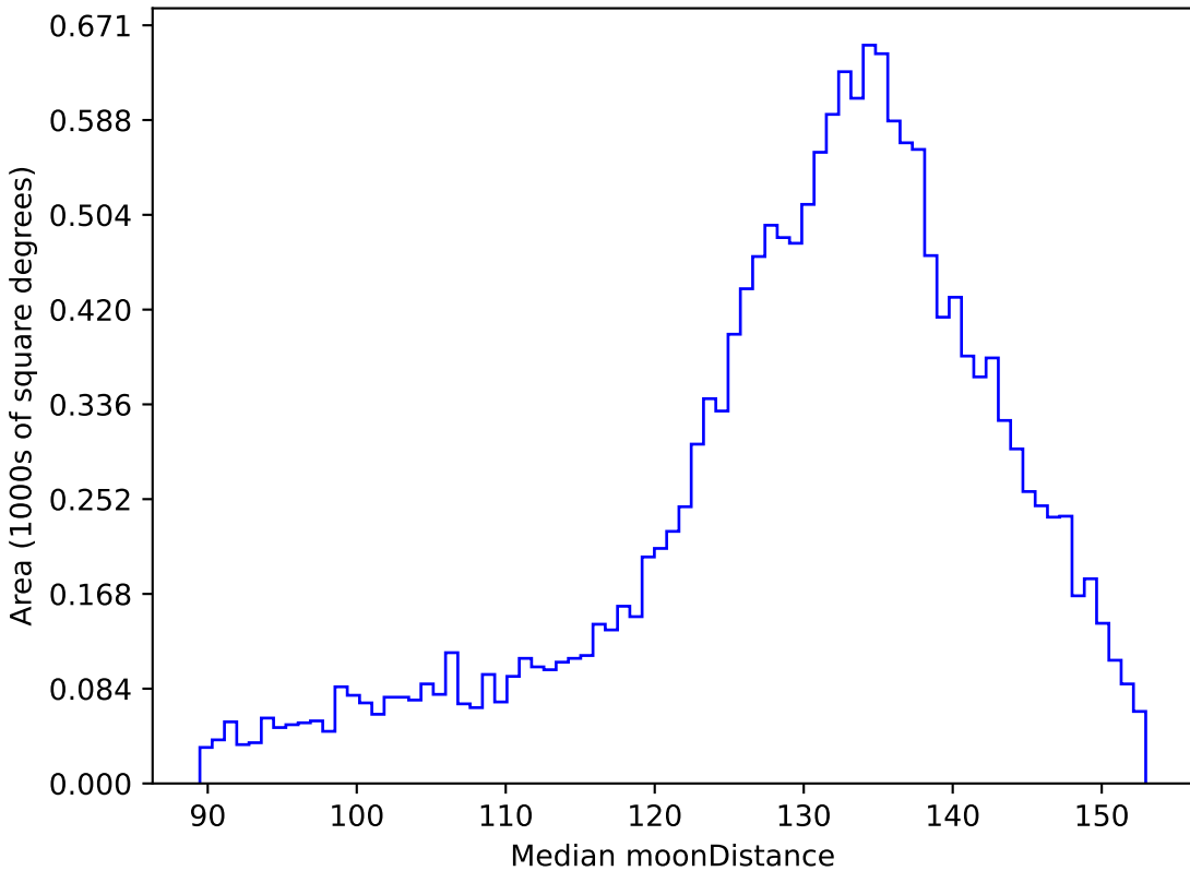
baseline_v2.0_10yrs WFD u band: Median moonDistance
