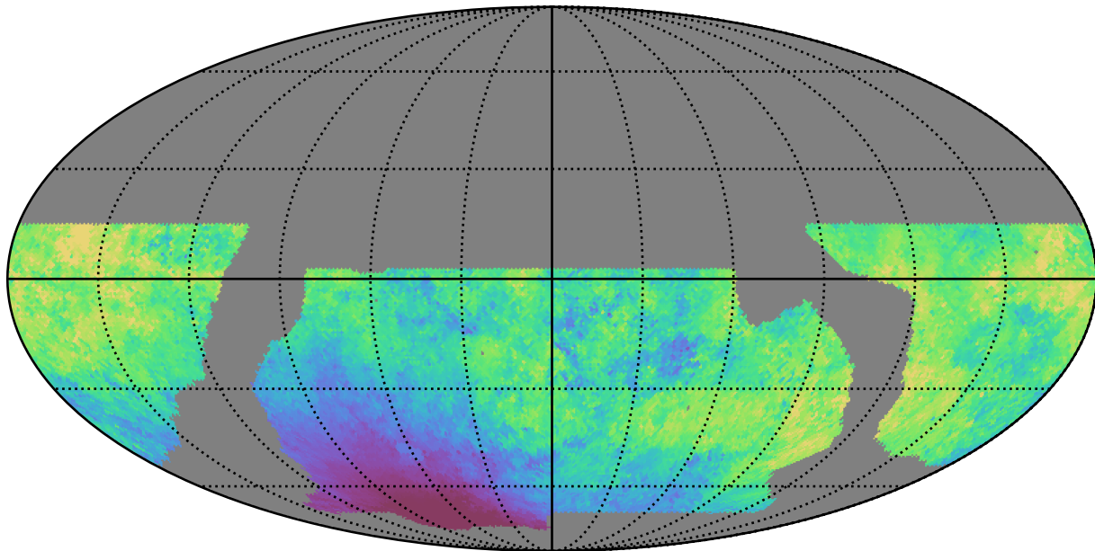
baseline_v2.0_10yrs WFD r band: Median moonDistance
