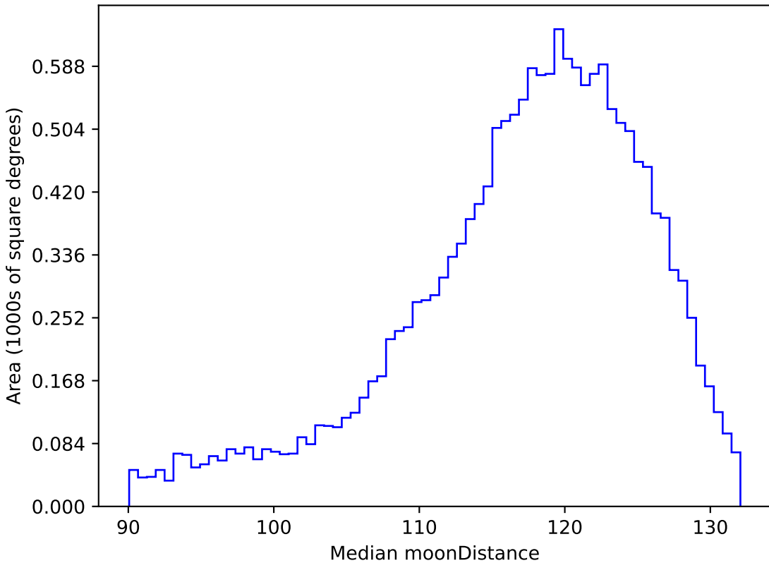
baseline_v2.0_10yrs WFD r band: Median moonDistance
