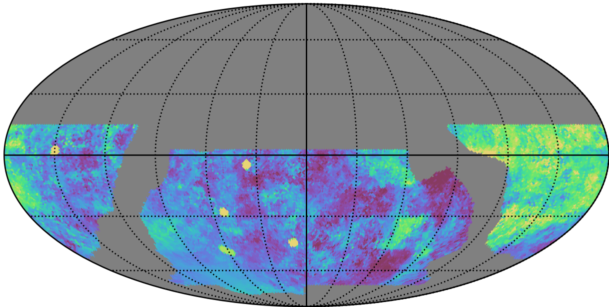
baseline_v2.0_10yrs WFD i band: Median moonDistance
