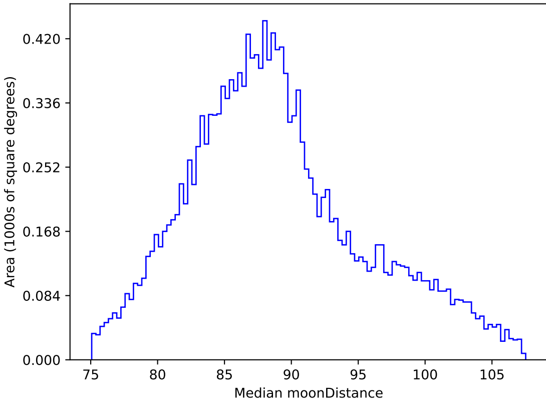
baseline_v2.0_10yrs WFD i band: Median moonDistance
