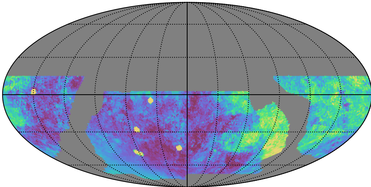
baseline_v2.0_10yrs WFD all bands: Median moonDistance
