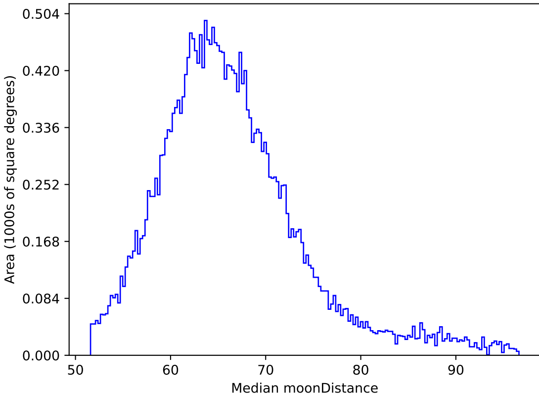
baseline_v2.0_10yrs All sky z band: Median moonDistance
