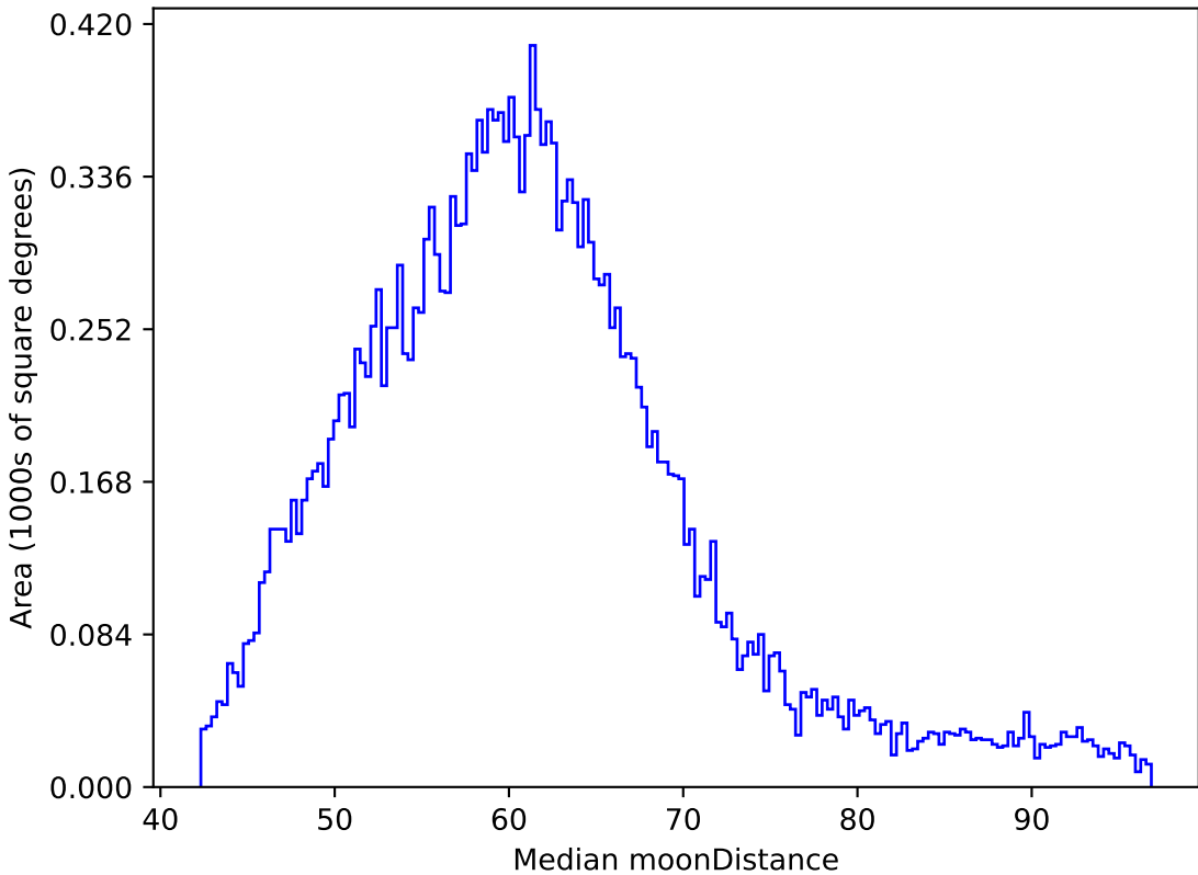
baseline_v2.0_10yrs All sky y band: Median moonDistance
