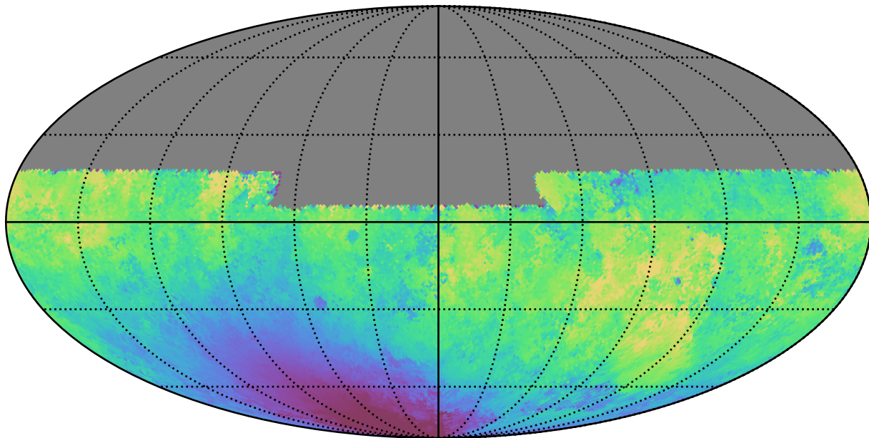
baseline_v2.0_10yrs All sky u band: Median moonDistance
