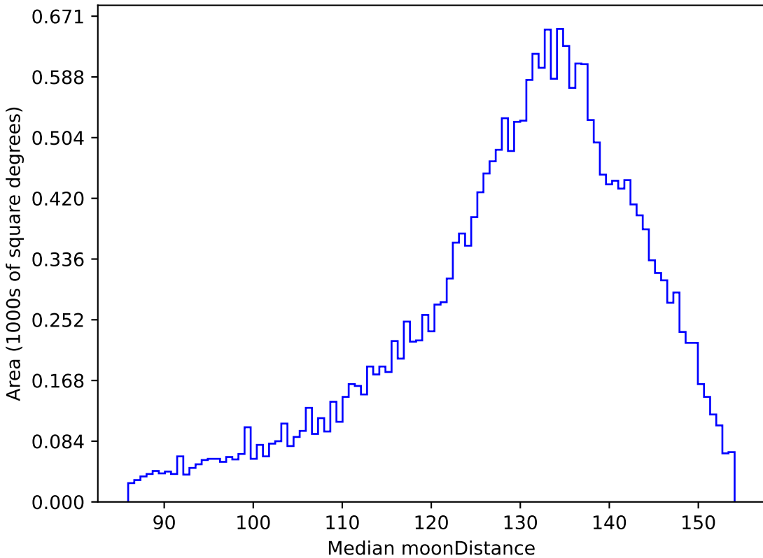
baseline_v2.0_10yrs All sky u band: Median moonDistance
