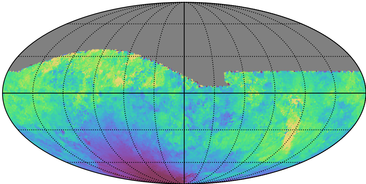
baseline_v2.0_10yrs All sky r band: Median moonDistance
