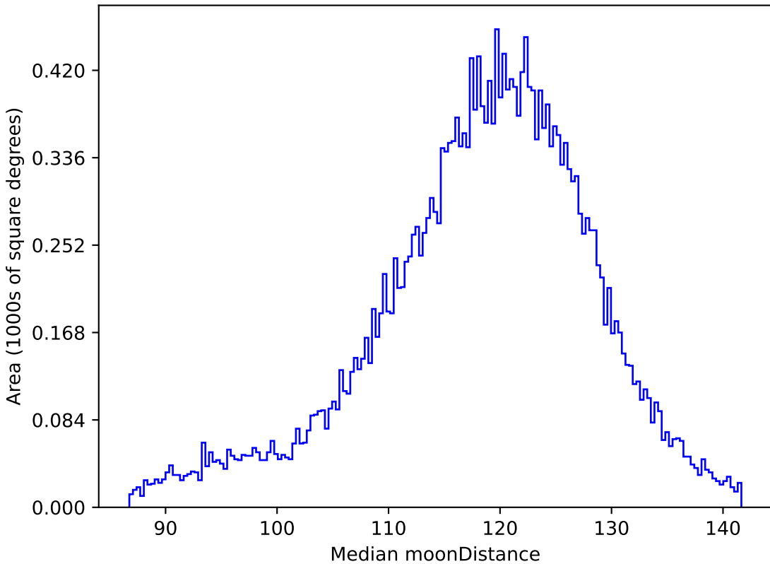
baseline_v2.0_10yrs All sky r band: Median moonDistance
