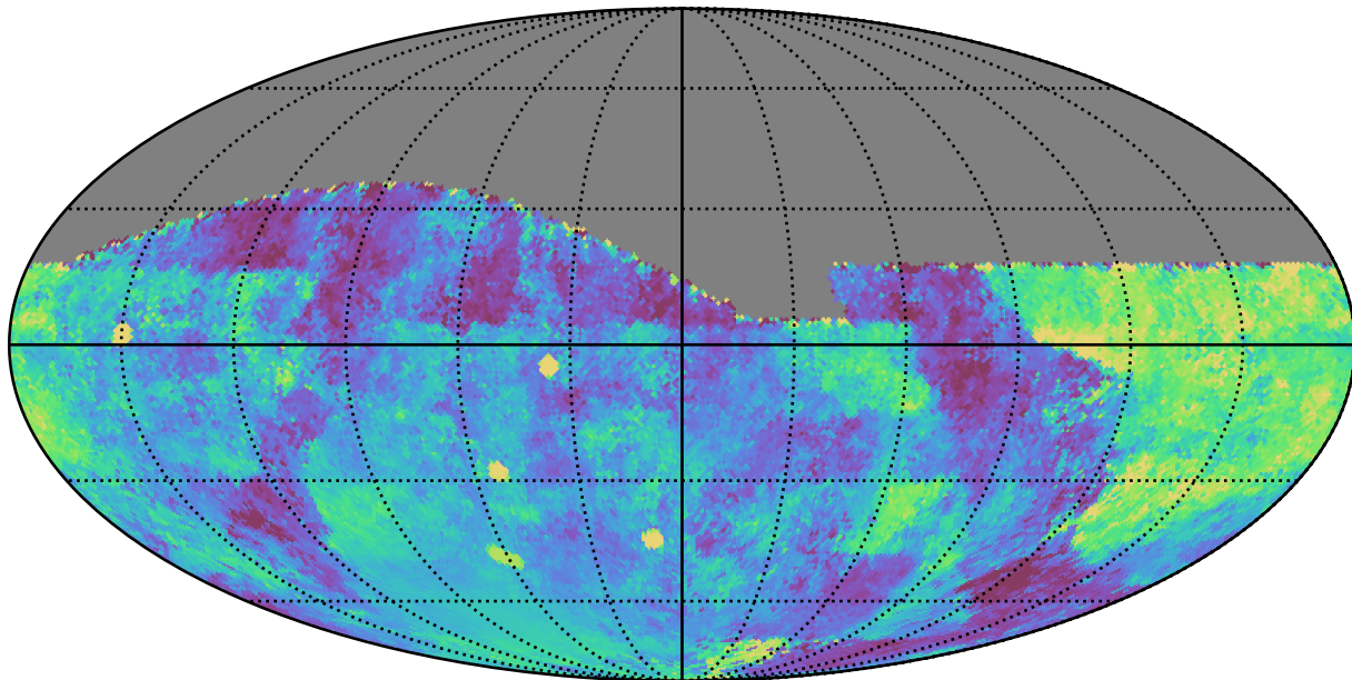
baseline_v2.0_10yrs All sky i band: Median moonDistance
