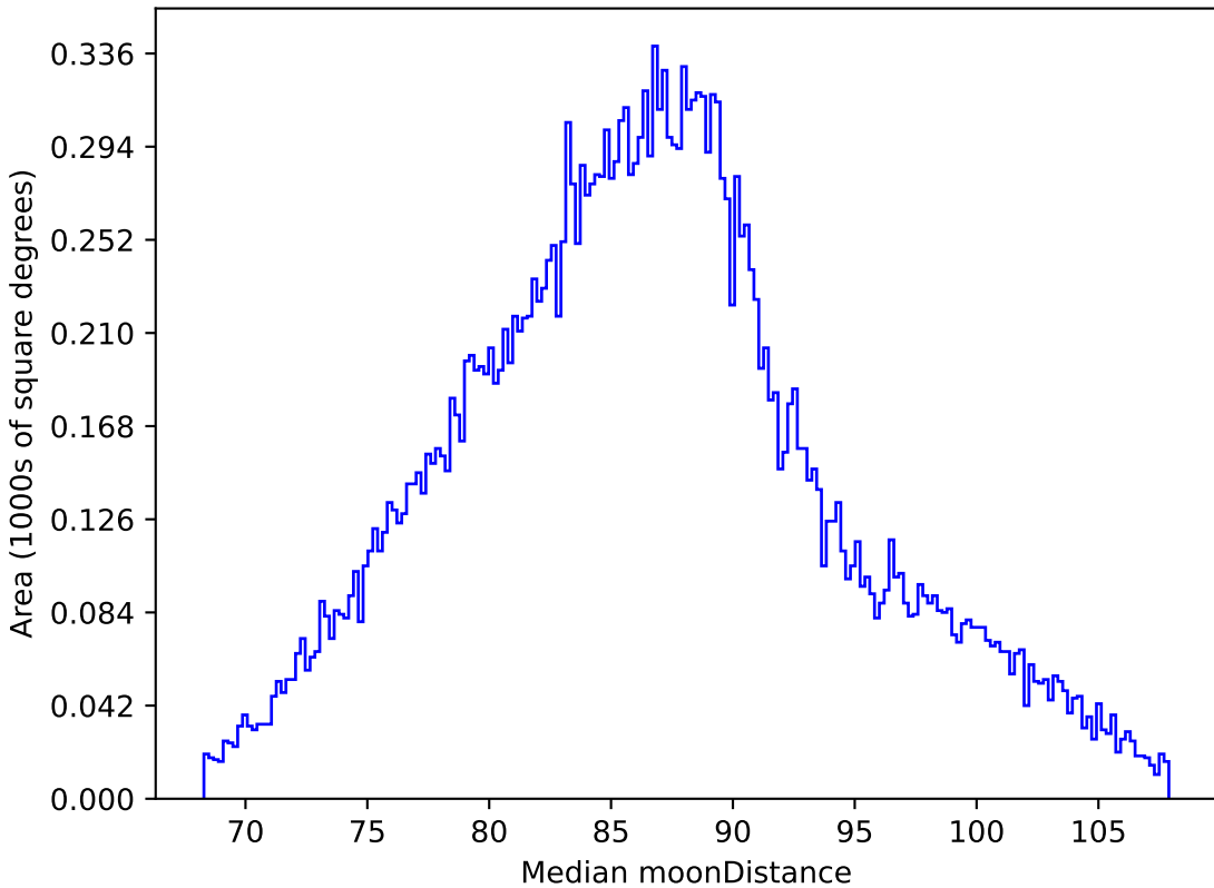
baseline_v2.0_10yrs All sky i band: Median moonDistance
