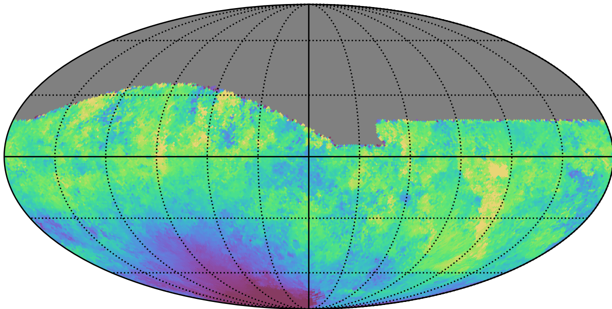
baseline_v2.0_10yrs All sky g band: Median moonDistance
