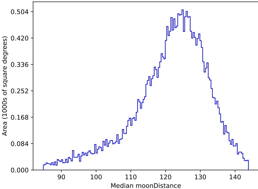
baseline_v2.0_10yrs All sky g band: Median moonDistance
